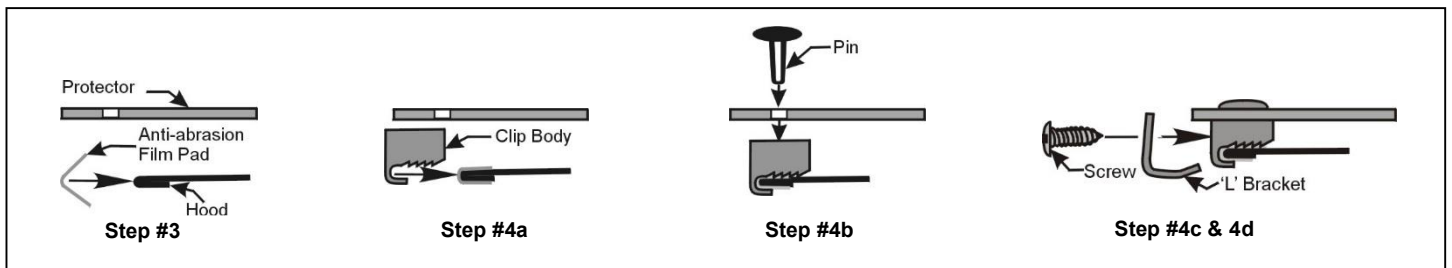
Illustration #2– Clip Configuration – Patent No. 6,892,427
