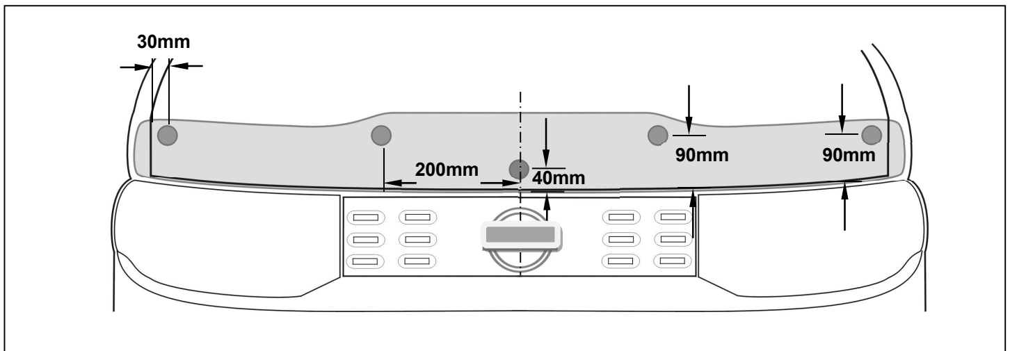
Illustration #1 – Bumpons Placement
